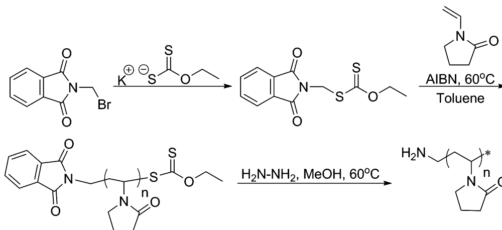
Scheme 1. Synthesis of PVP using O -ethyl- S -(phthalimidylmethyl) xanthate as a RAFT agent and subsequent removal of phthalimide functionality to afford amine-functionalized polymer chains.
