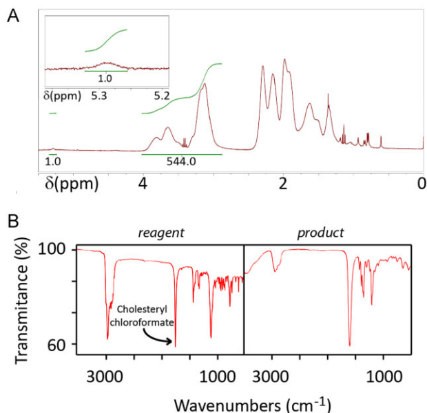
Figure 2. A) ^1\text{H} NMR and B) FT-IR characterization of cholesterol conjugation to amine-functionalized PVP through carbamate linkages.
